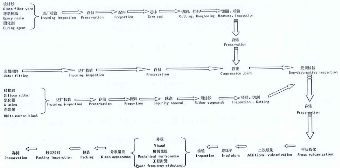
QUALITY CONTROL FLOW CHART FOR MANUFACTURING PROCESS OF INSULATOR
